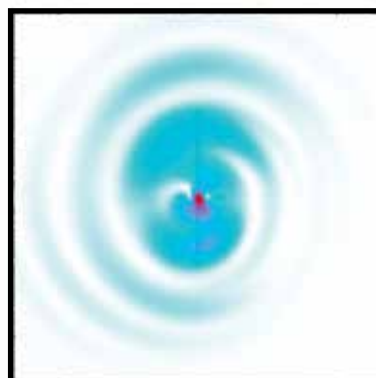
The Spinning Electron
